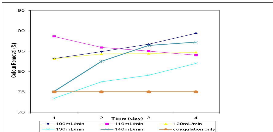
Figure 4. Colour Removal versus Time at Different Filtration Rates by Using 5µm PP and pH7.5
