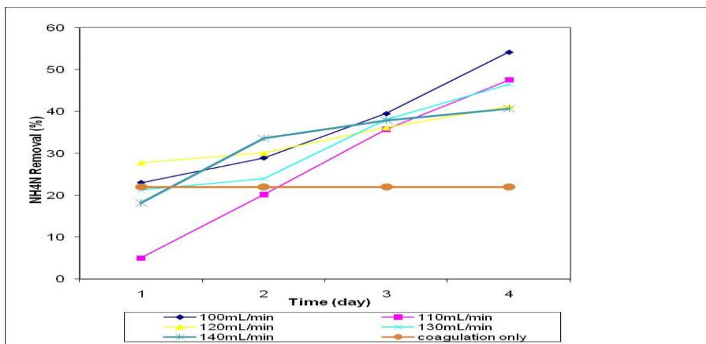
Figure 6. \text{NH}_4\text{N} Removal versus Time for Different Filtration Rates by using 5 \mu\text{m} PP and pH7.5
