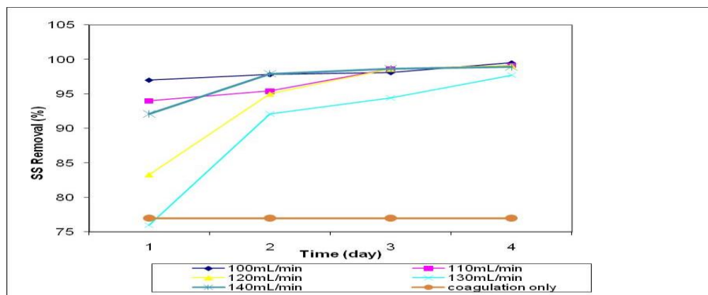
Figure 5. Suspended Solids (SS) Removal versus Time at Different Filtration Rates by using 5µm PP and pH7.5
